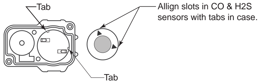
Figure 8: Replacing the Sensor
