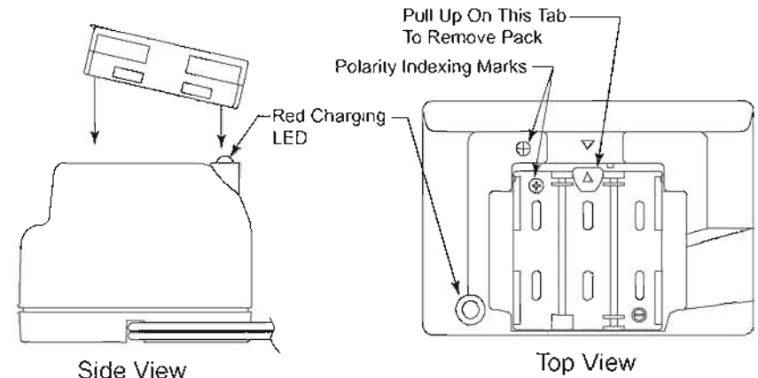
Figure 7: Putting the Battery Pack into the Charging Station
