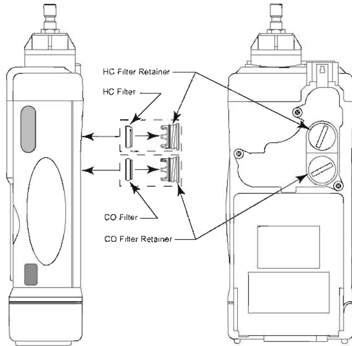
Figure 8: Replacing the CO and HC Filters
