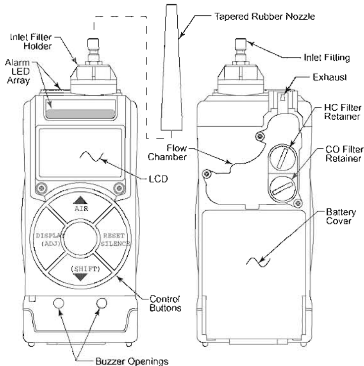
Figure 1: Components of the GX-2003, Front & Back
