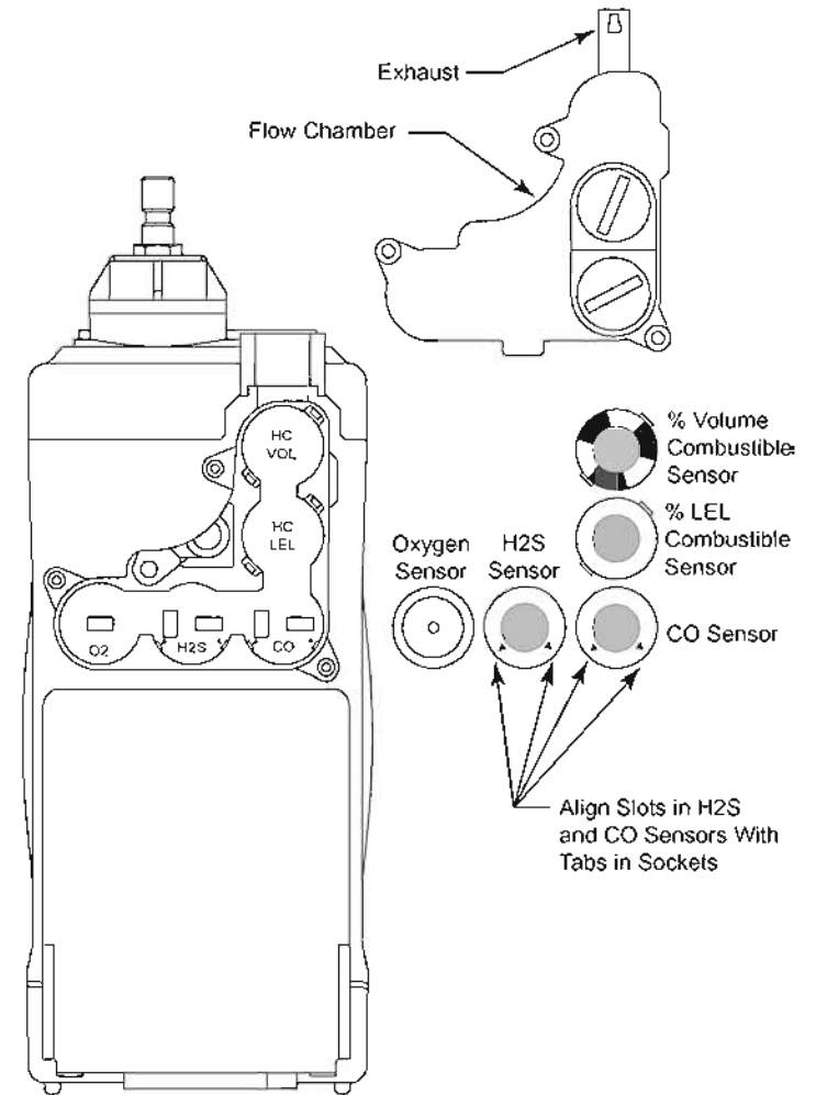
Figure 9: Replacing a Sensor
