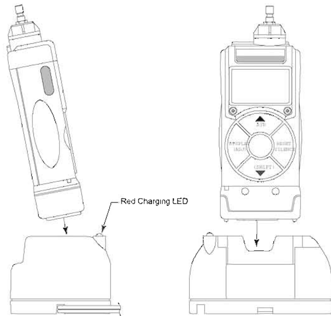
Figure 6: Putting the GX-2003 into the Charging Station
