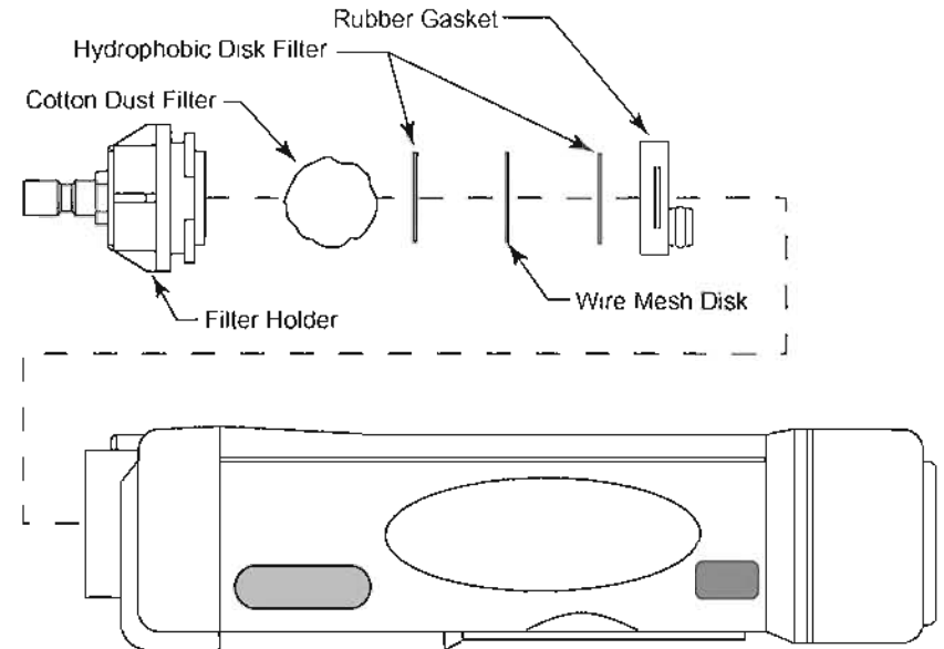
Figure 10: Changing the Filters & Wire Mesh Disk
