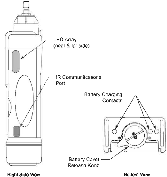
Figure 2 : Components of the GX-2003, Side & Bottom
